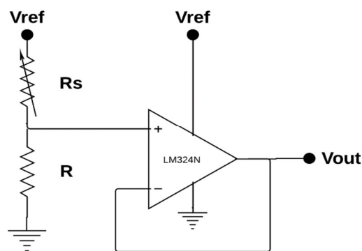
Figure 4 - Conditioning circuit for force sensors (RS-sensor resistance, R-reference resistance)
